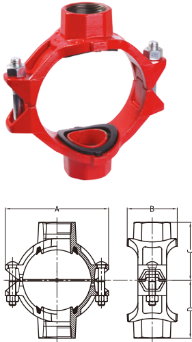
Mechanical Cross Threaded Outlet
