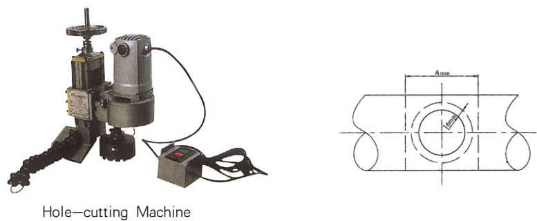
Hole-cutting Machine
