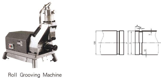
Roll Grooving Machine
